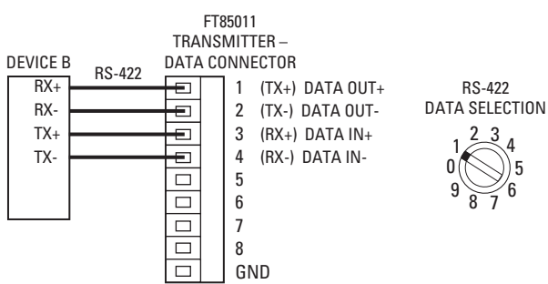
RS-422 DATA CONNECTIONS BETWEEN DEVICE B AND FT85011 TRANSMITTER
